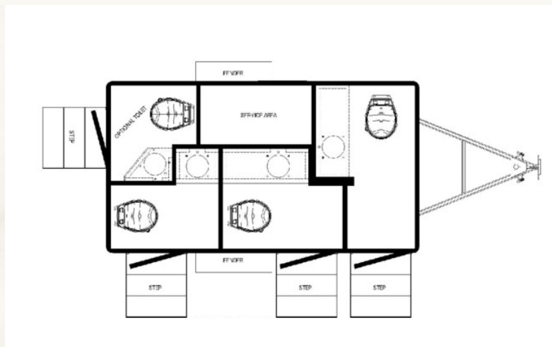
FLOORPLAN
